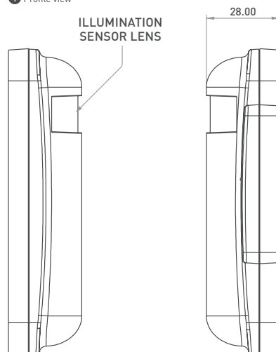
FIGURE 1 Dimensions (unit: mm)
