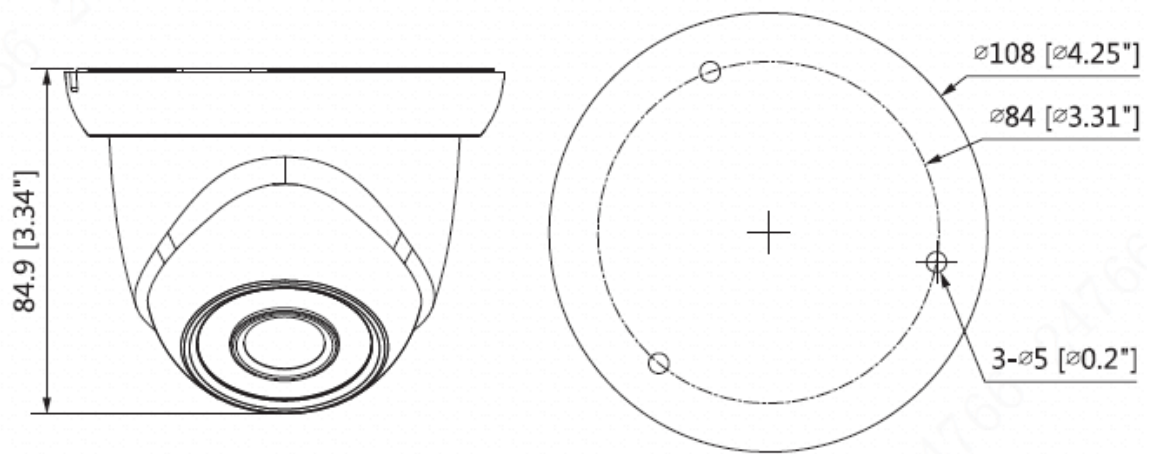
Figure 1-2 Dimensions
