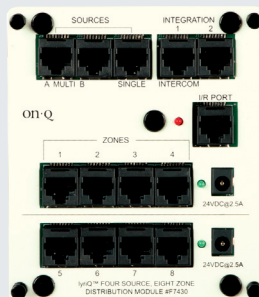
F7430 Four Source, Eight Zone Distribution Module
