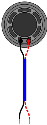
SINGLE SUBWOOFER This solution will yield a 4-ohm load. Connect to the outputs of the amplifier.
