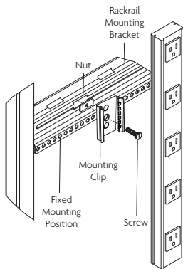
Rack-Mounting the PDU 16
