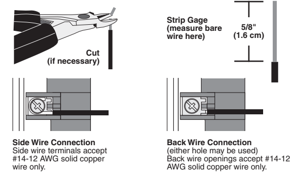
Dual Controlled Outlets
