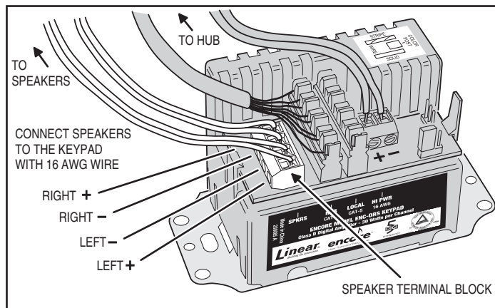
Figure 17. Speaker Connections
