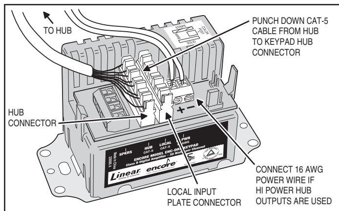
Figure 15. Keypad Connections
