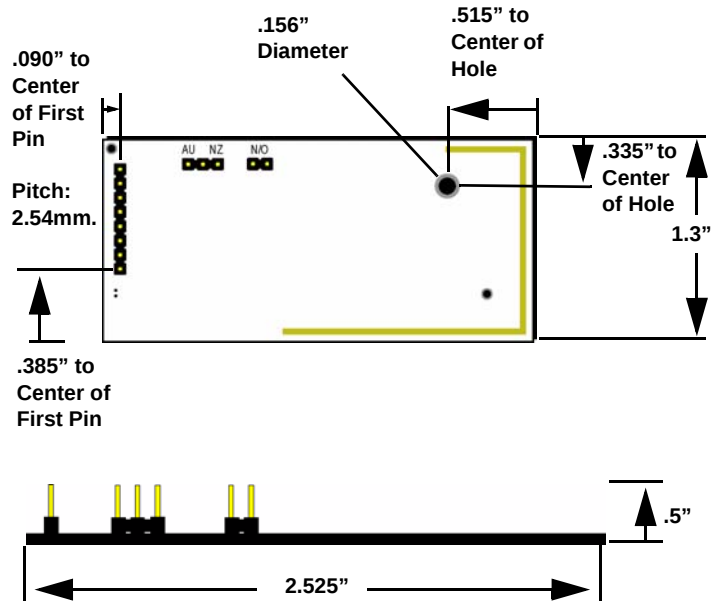
Figure 4 E*1941 One-Way Binary RF Module Dimensions
