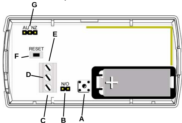
Figure 1 EN1212 components
