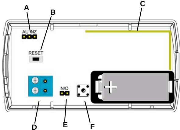
Figure 1 EN1210EOL components
