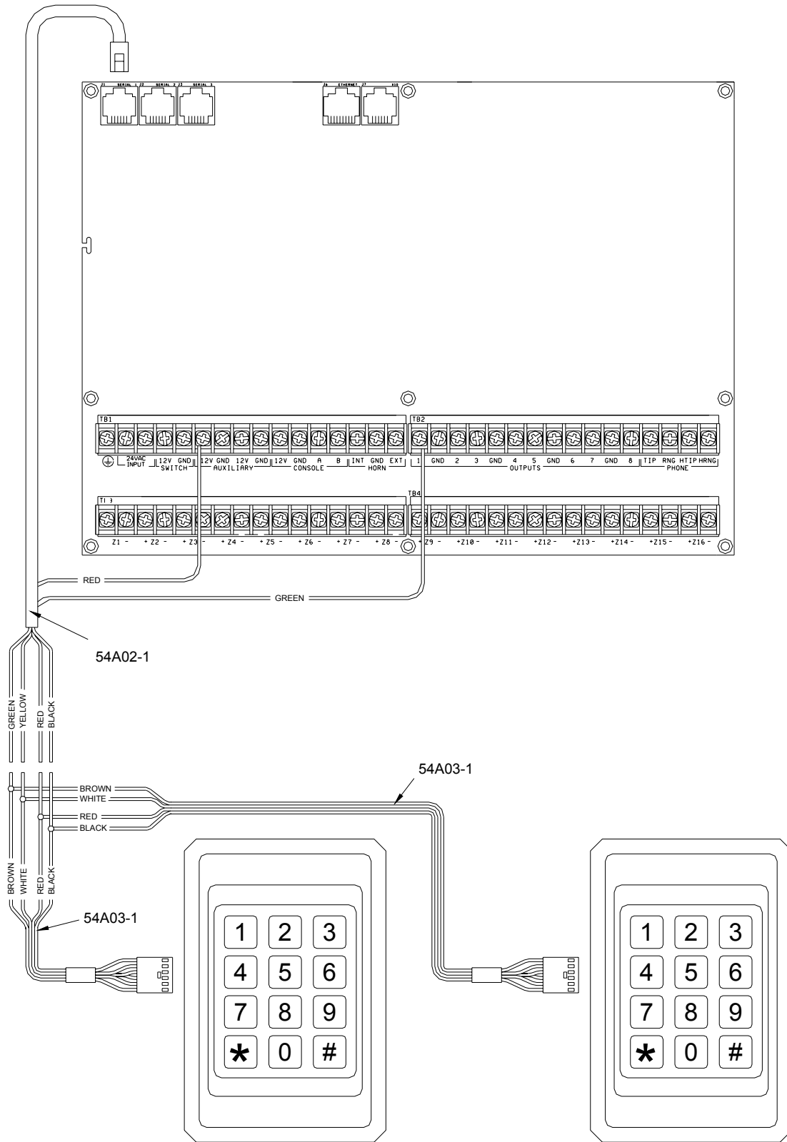
FIGURE 1 – MODEL 54A00-1 CONNECTIONS
