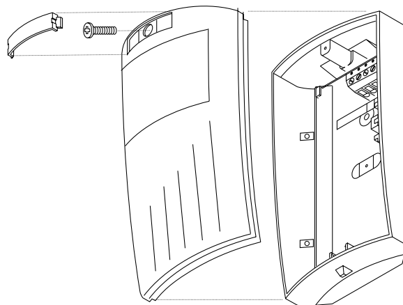
Figure 1. Sensor (exploded)
