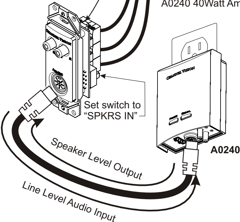
B-Speakers powered by A0240 40Watt Amplifier
